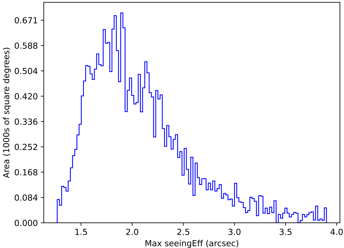
too_ignore_100_4v3.4_10yrs Yr 1 all bands: Max seeingEff
