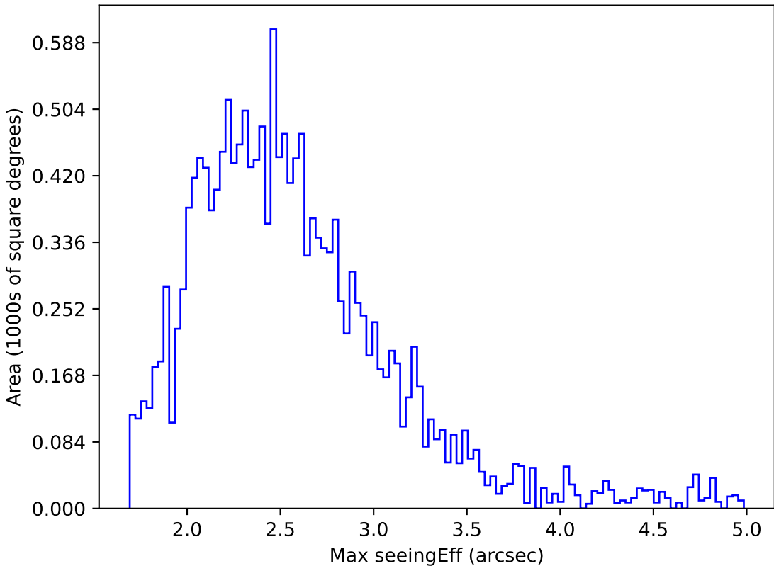
too_ignore_100_4v3.4_10yrs WFD z band: Max seeingEff
