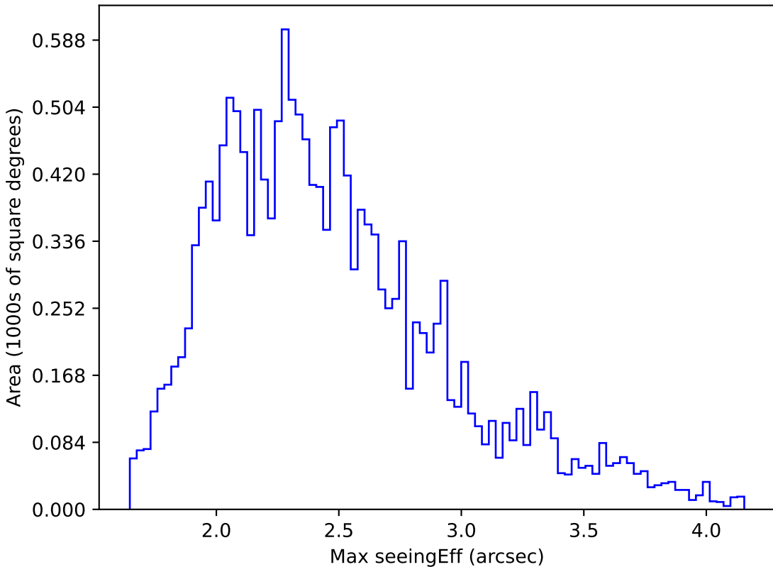
too_ignore_100_4v3.4_10yrs WFD u band: Max seeingEff
