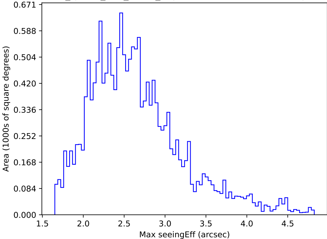
too_ignore_100_4v3.4_10yrs WFD i band: Max seeingEff
