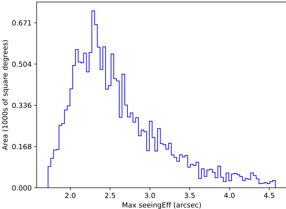
too_ignore_100_4v3.4_10yrs WFD g band: Max seeingEff
