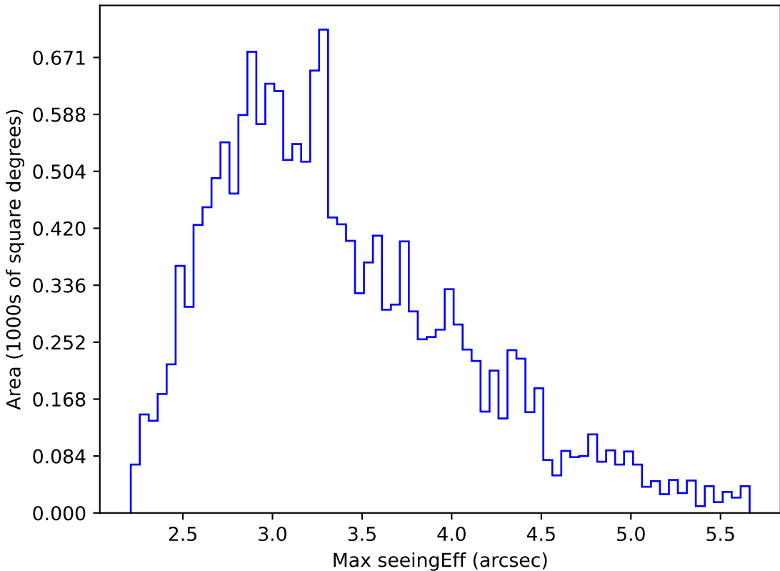
too_ignore_100_4v3.4_10yrs WFD all bands: Max seeingEff
