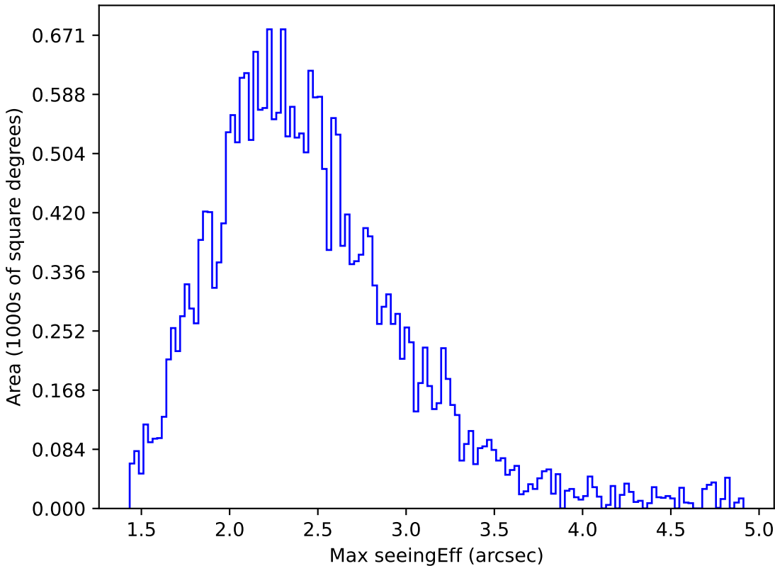
too_ignore_100_4v3.4_10yrs All sky z band: Max seeingEff
