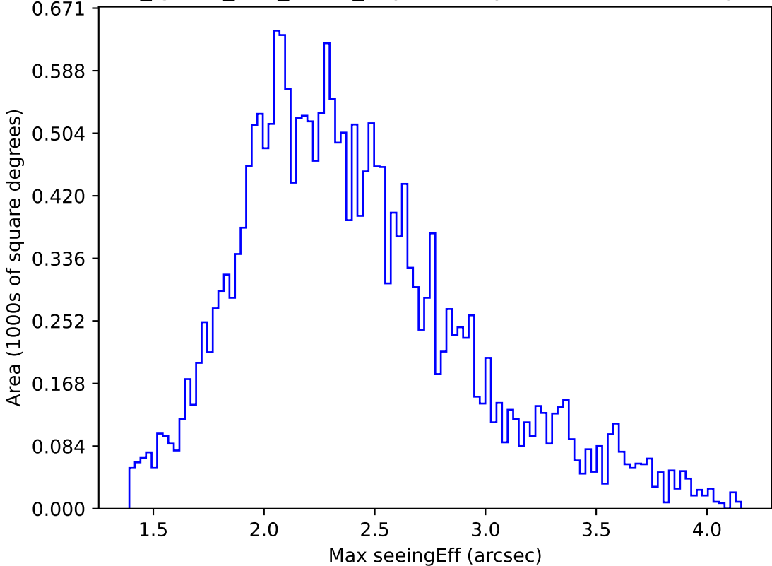
too_ignore_100_4v3.4_10yrs All sky u band: Max seeingEff
