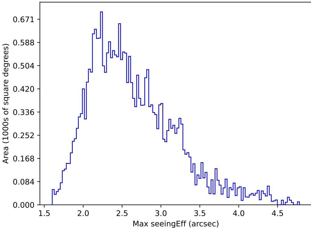
too_ignore_100_4v3.4_10yrs All sky r band: Max seeingEff
