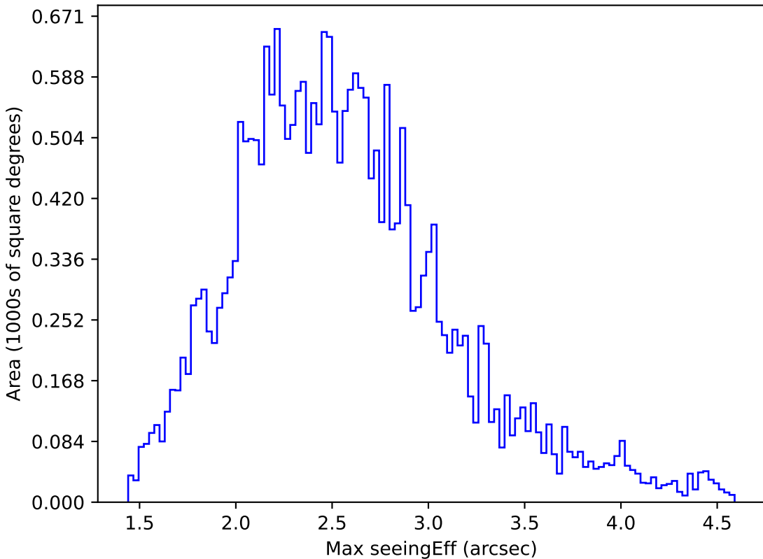
too_ignore_100_4v3.4_10yrs All sky i band: Max seeingEff
