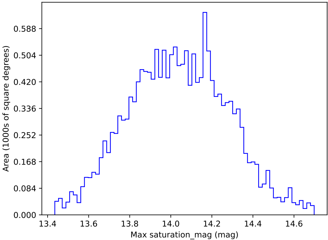
too_ignore_100_4v3.4_10yrs WFD u band: Max saturation_mag
