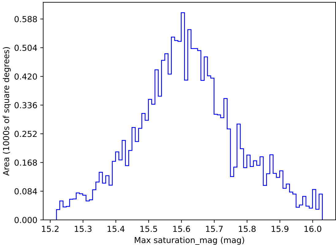
too_ignore_100_4v3.4_10yrs WFD i band: Max saturation_mag
