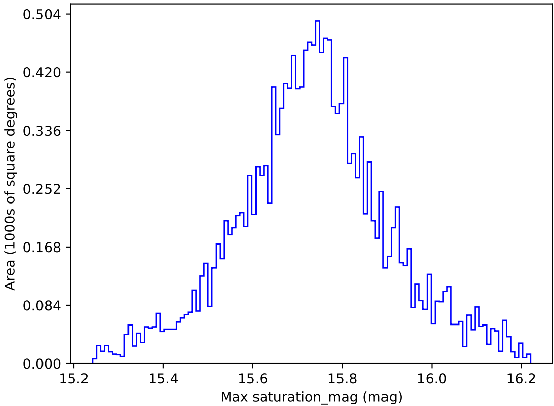
too_ignore_100_4v3.4_10yrs WFD g band: Max saturation_mag
