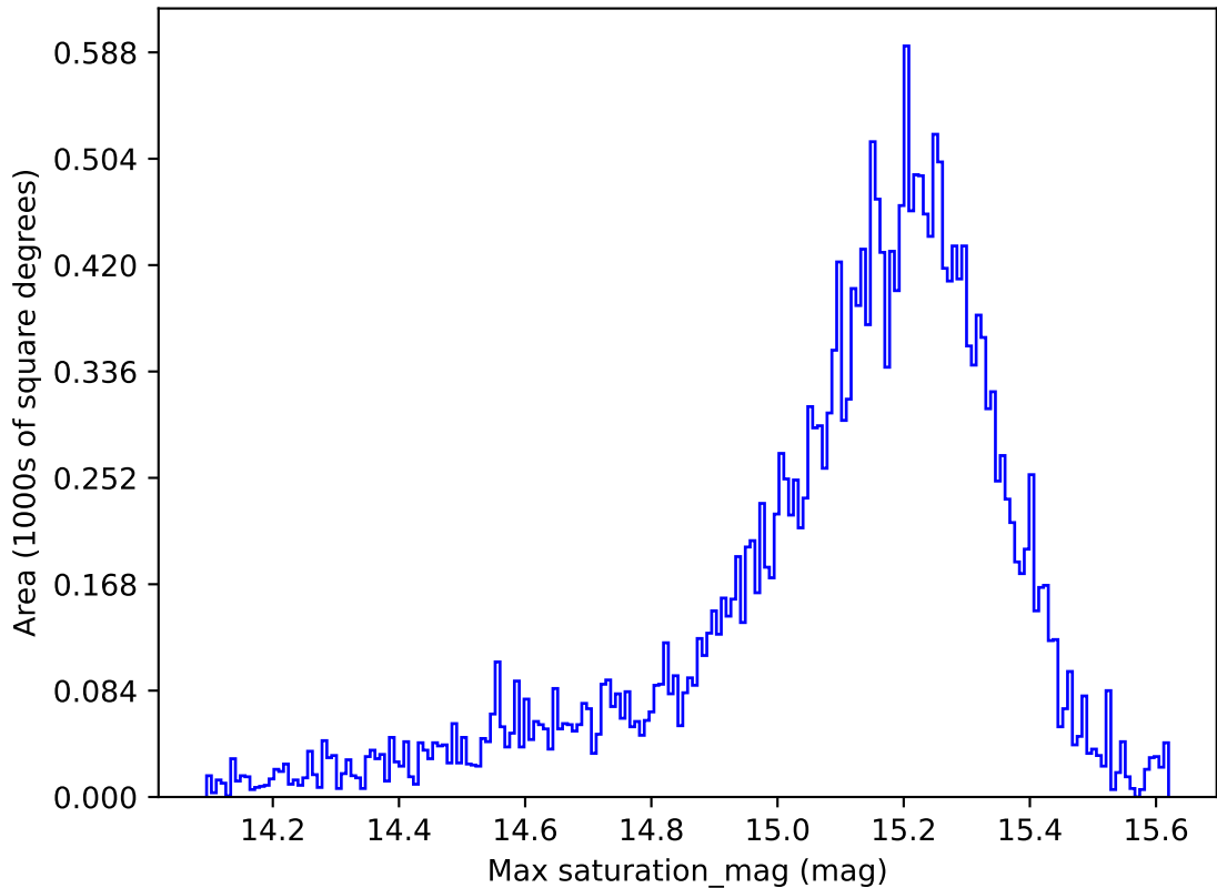
too_ignore_100_4v3.4_10yrs All sky z band: Max saturation_mag
