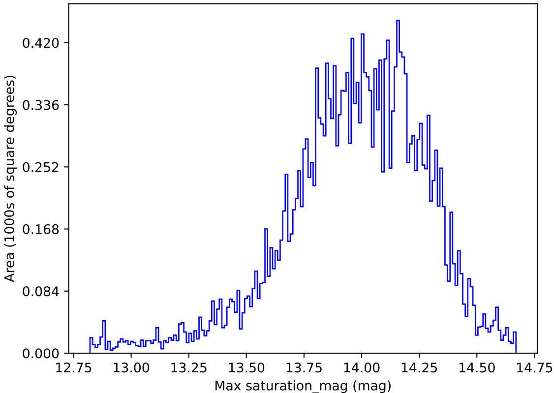
too_ignore_100_4v3.4_10yrs All sky u band: Max saturation_mag
