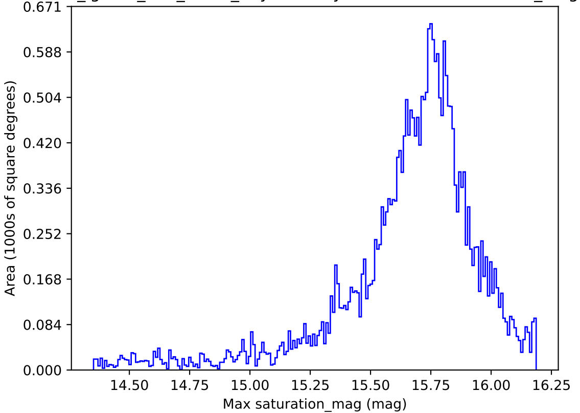
too_ignore_100_4v3.4_10yrs All sky r band: Max saturation_mag
