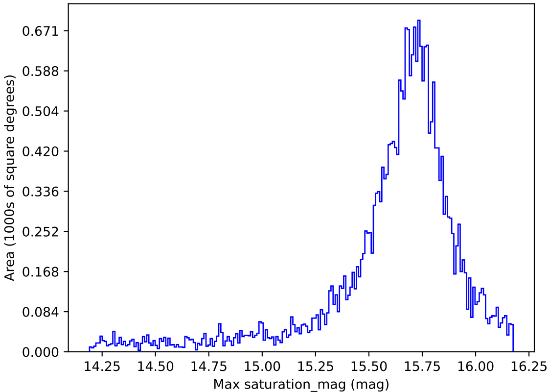
too_ignore_100_4v3.4_10yrs All sky g band: Max saturation_mag
