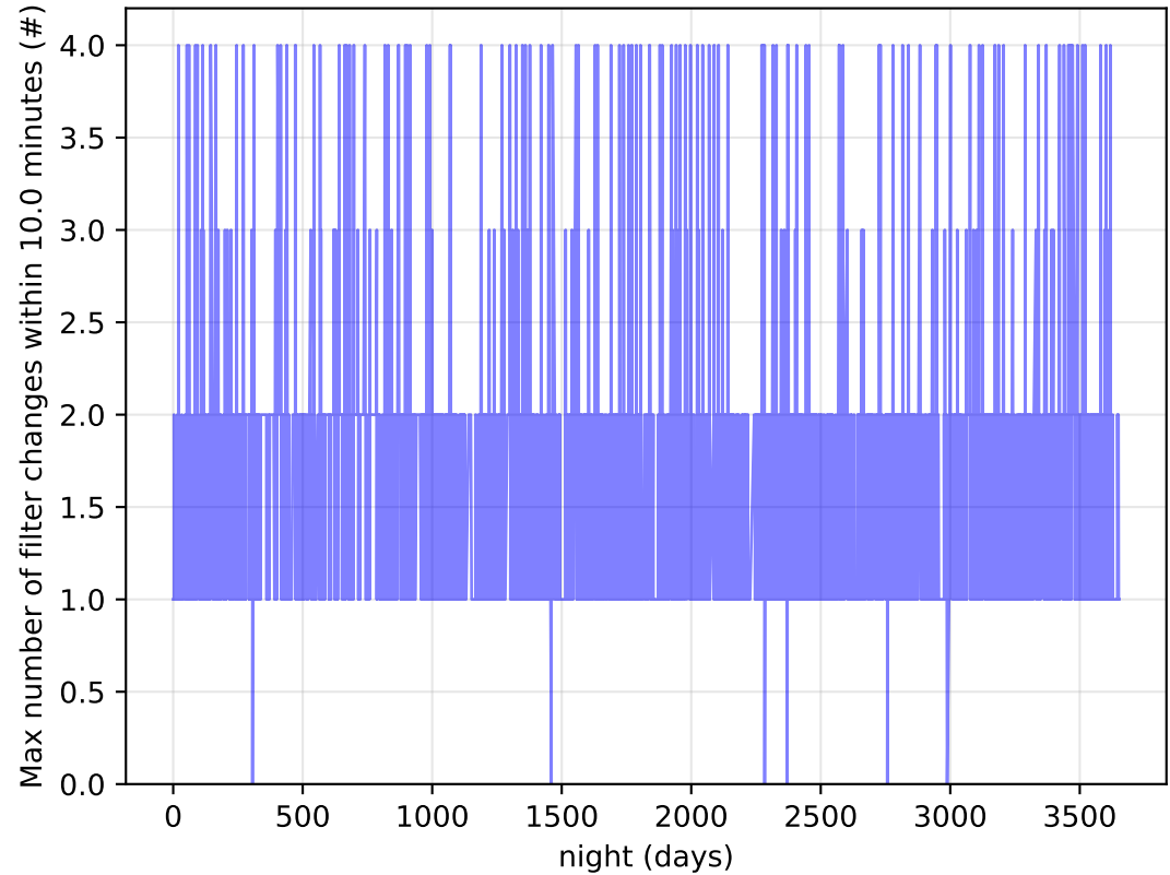
too_ignore_100_4v3.4_10yrs Per Night: Max number of filter changes within 10.0 minutes
