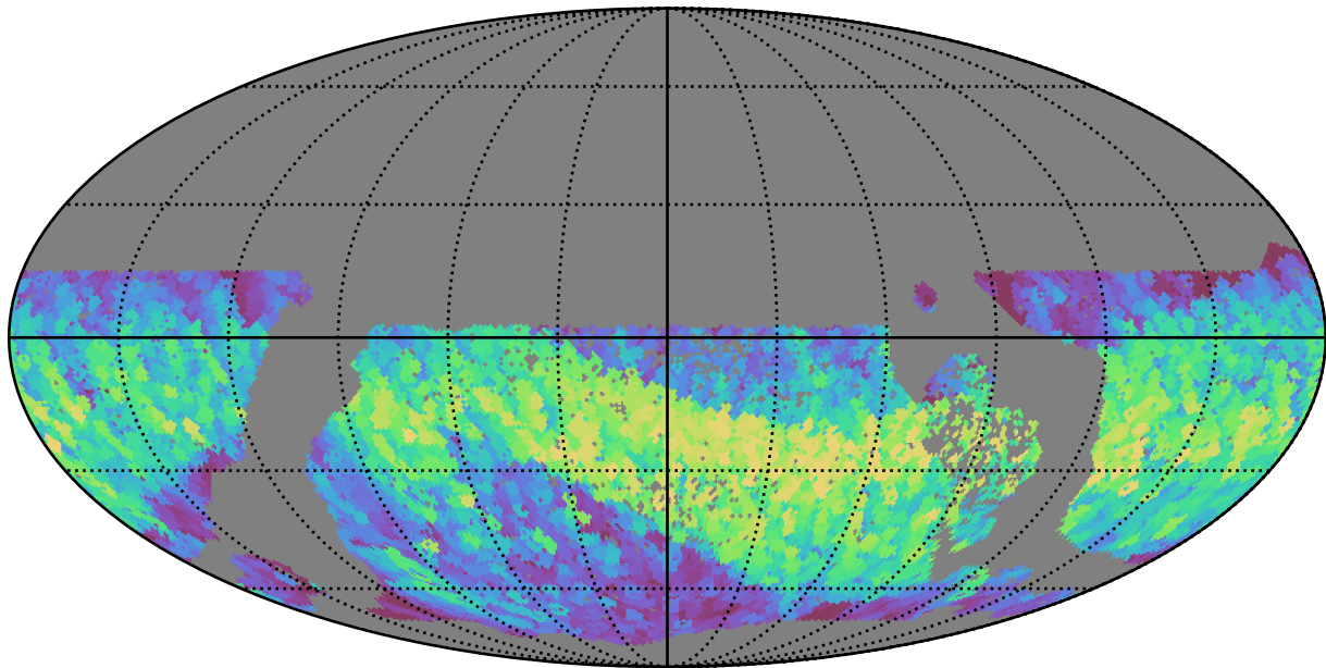
too_ignore_100_4v3.4_10yrs WFD z band: Max normairmass
