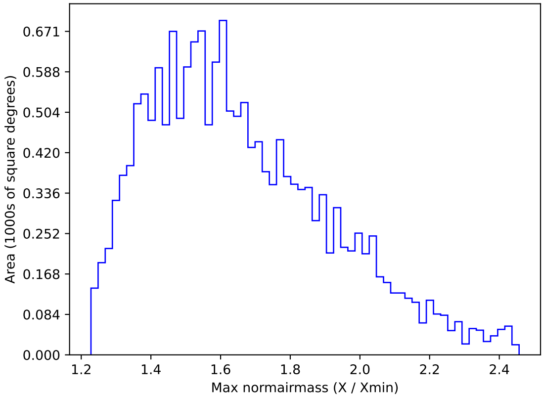
too_ignore_100_4v3.4_10yrs WFD u band: Max normairmass
