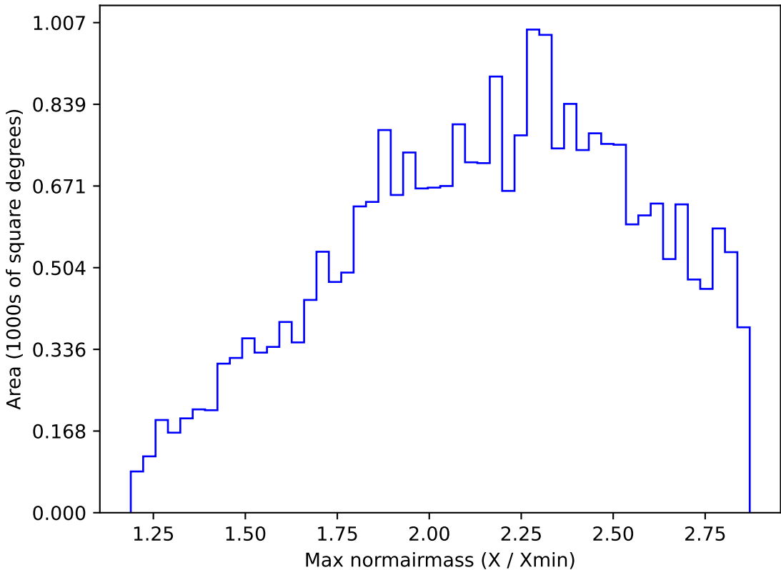
too_ignore_100_4v3.4_10yrs All sky z band: Max normairmass
