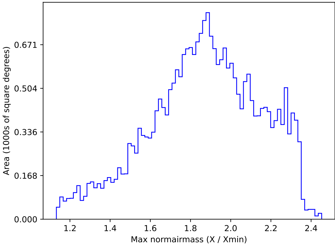
too_ignore_100_4v3.4_10yrs All sky g band: Max normairmass
