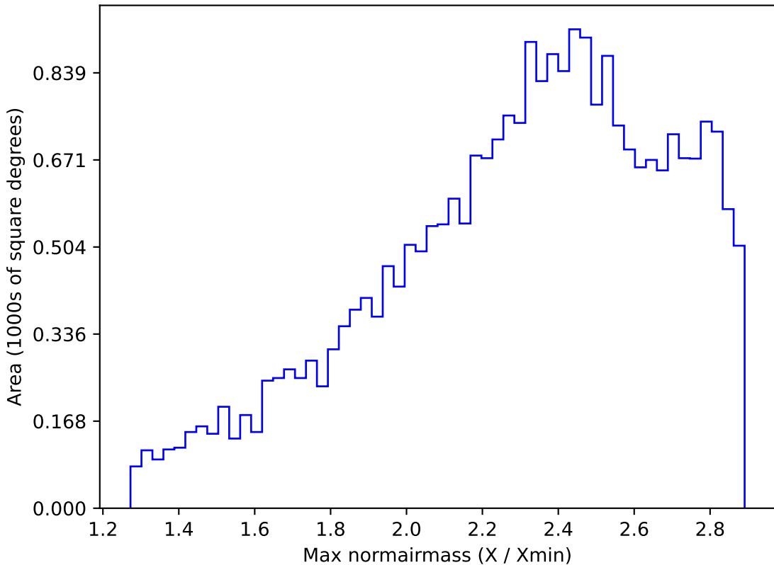
too_ignore_100_4v3.4_10yrs All sky all bands: Max normairmass
