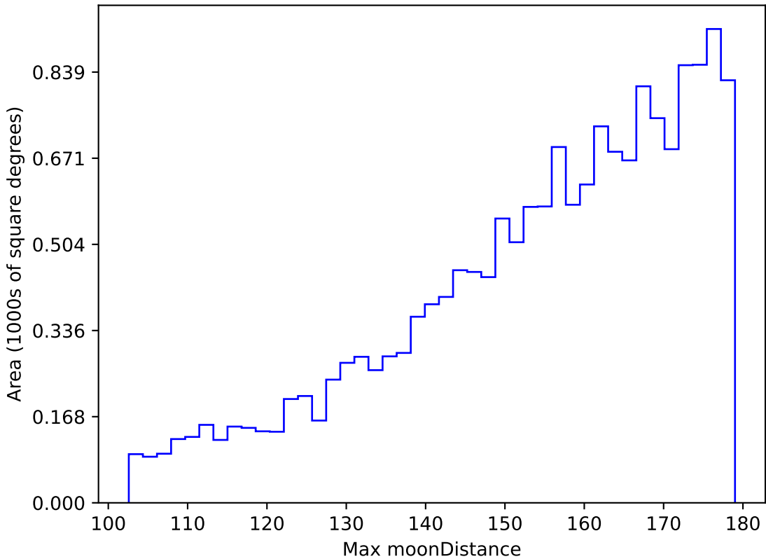
too_ignore_100_4v3.4_10yrs WFD u band: Max moonDistance
