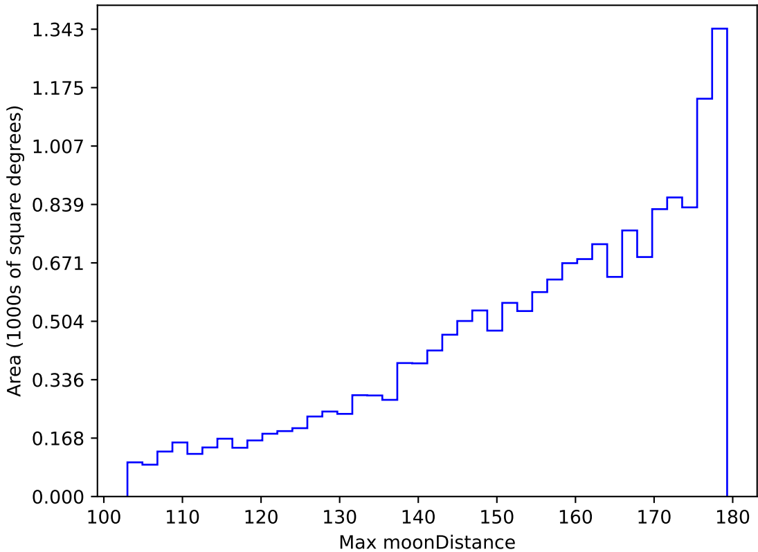
too_ignore_100_4v3.4_10yrs WFD i band: Max moonDistance
