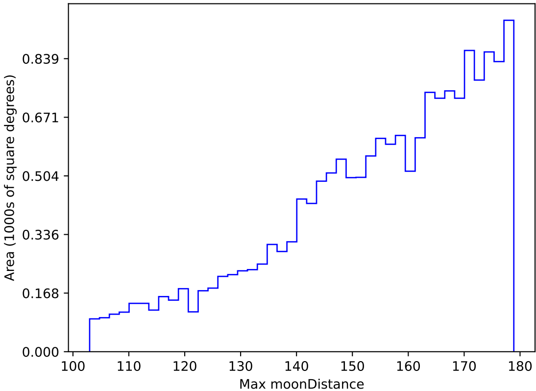
too_ignore_100_4v3.4_10yrs WFD g band: Max moonDistance
