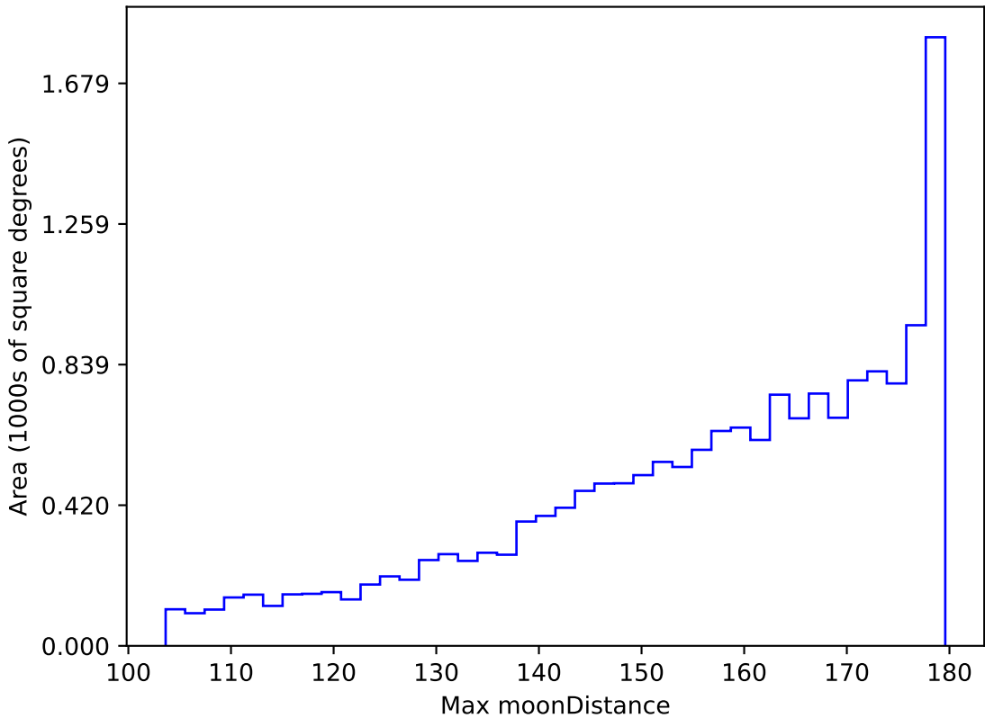
too_ignore_100_4v3.4_10yrs WFD all bands: Max moonDistance
