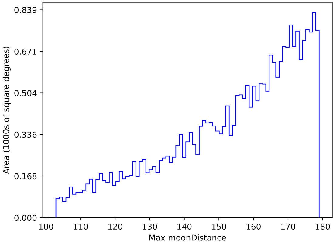
too_ignore_100_4v3.4_10yrs All sky z band: Max moonDistance
