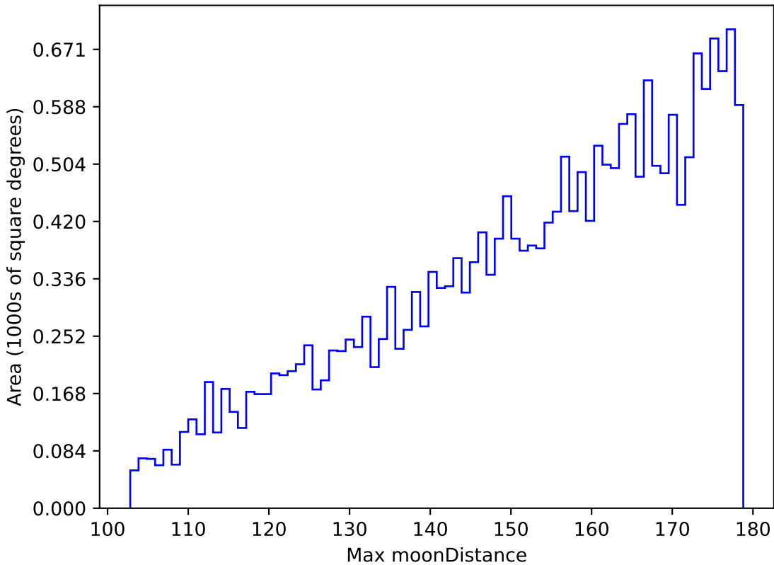
too_ignore_100_4v3.4_10yrs All sky u band: Max moonDistance
