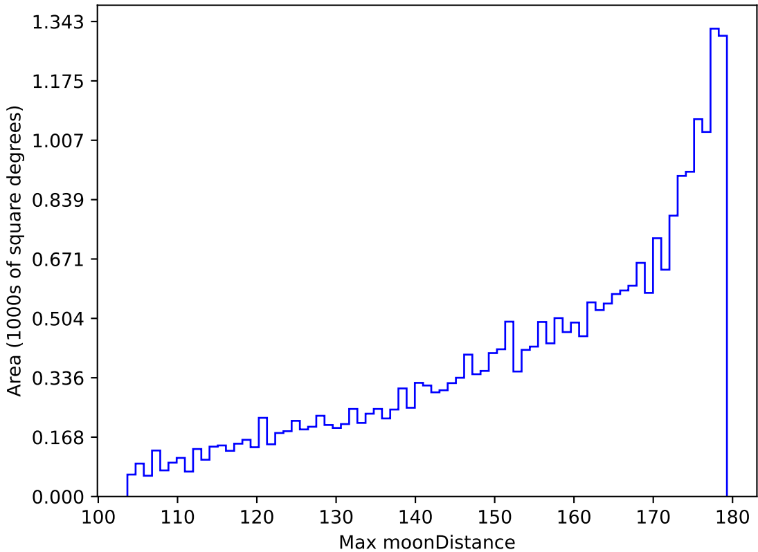
too_ignore_100_4v3.4_10yrs All sky r band: Max moonDistance
