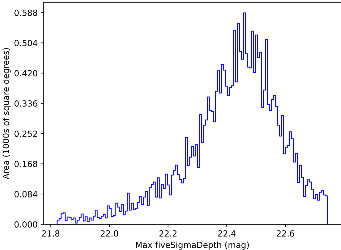
too_ignore_100_4v3.4_10yrs Yr 1 y band: Max fiveSigmaDepth
