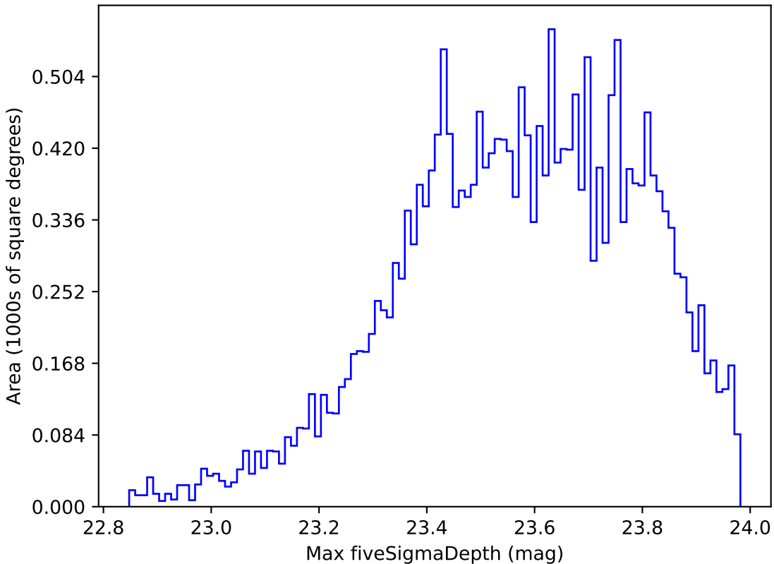
too_ignore_100_4v3.4_10yrs Yr 1 u band: Max fiveSigmaDepth
