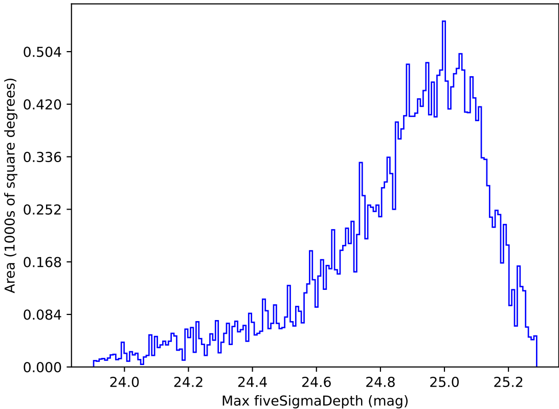
too_ignore_100_4v3.4_10yrs Yr 1 g band: Max fiveSigmaDepth
