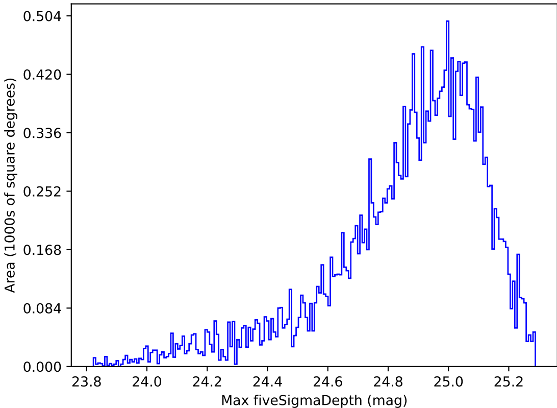
too_ignore_100_4v3.4_10yrs Yr 1 all bands: Max fiveSigmaDepth
