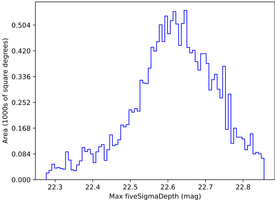
too_ignore_100_4v3.4_10yrs WFD y band: Max fiveSigmaDepth
