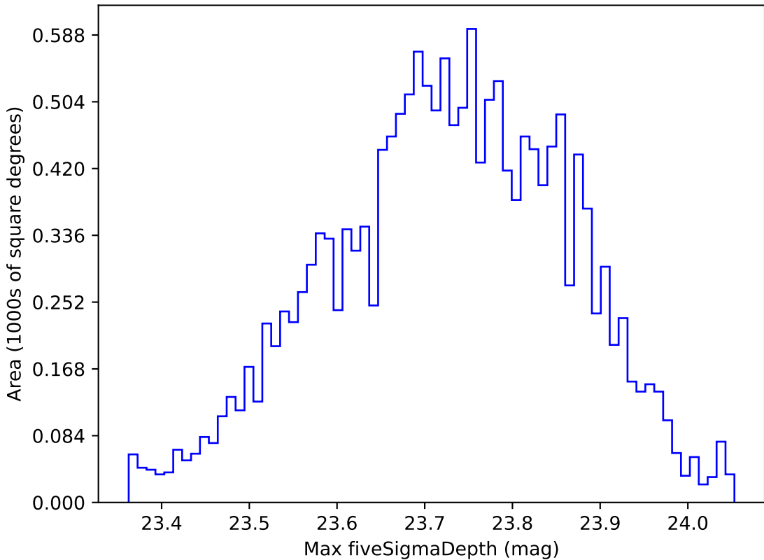
too_ignore_100_4v3.4_10yrs WFD u band: Max fiveSigmaDepth
