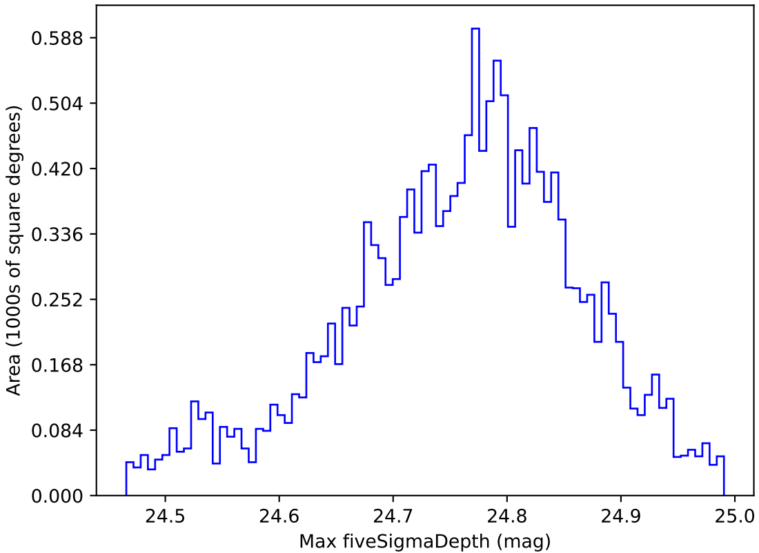
too_ignore_100_4v3.4_10yrs WFD r band: Max fiveSigmaDepth
