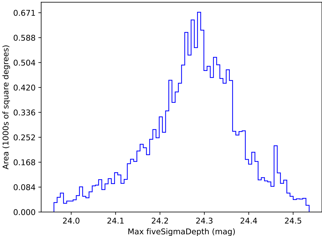
too_ignore_100_4v3.4_10yrs WFD i band: Max fiveSigmaDepth
