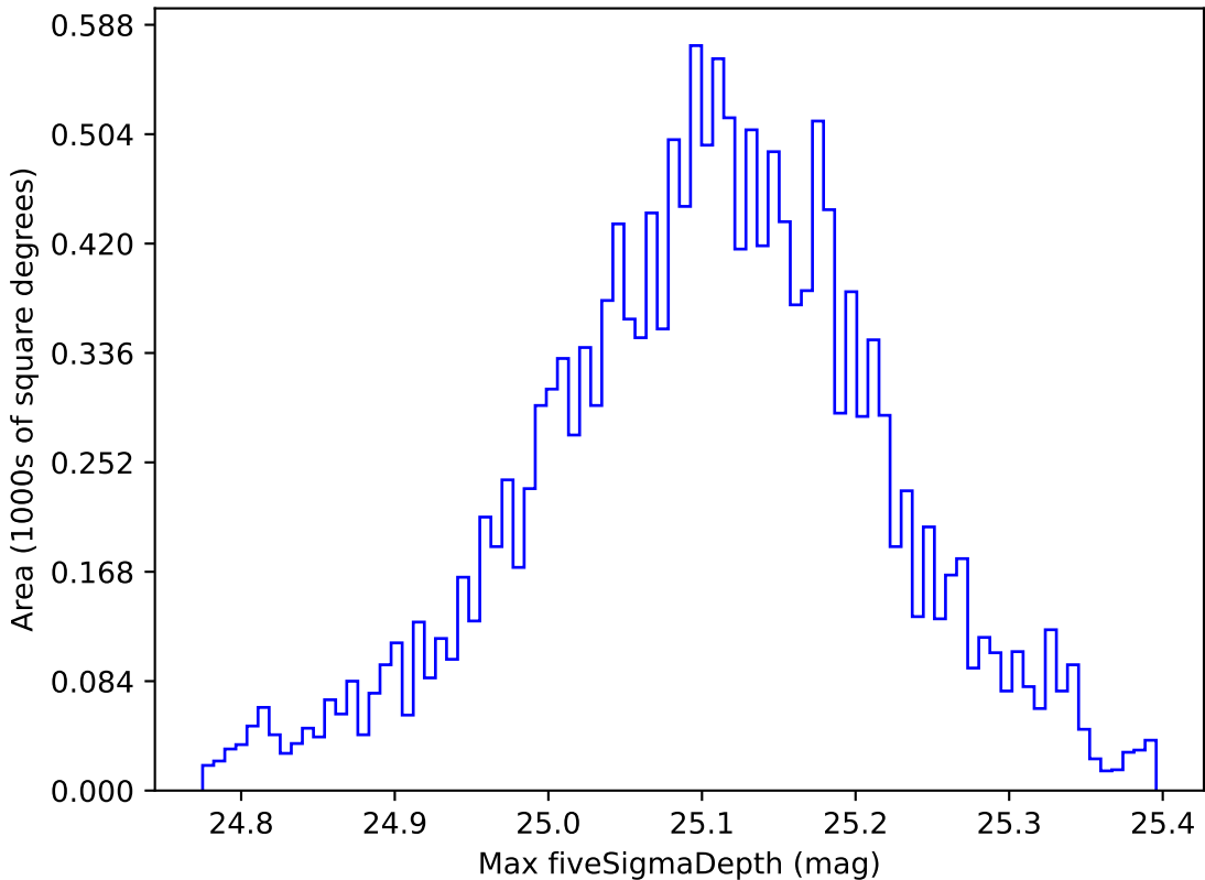
too_ignore_100_4v3.4_10yrs WFD g band: Max fiveSigmaDepth
