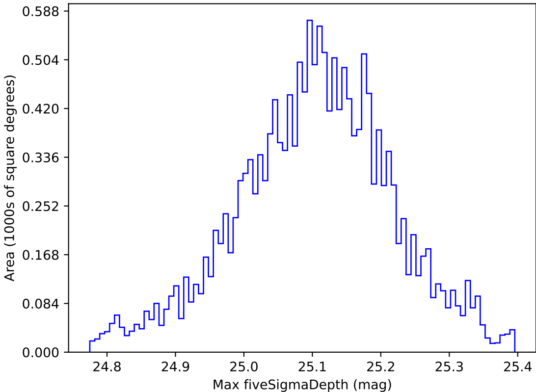
too_ignore_100_4v3.4_10yrs WFD all bands: Max fiveSigmaDepth
