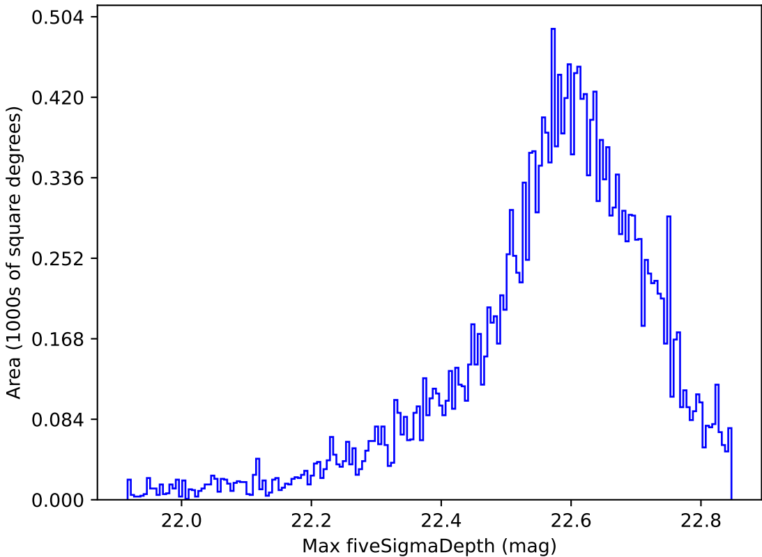
too_ignore_100_4v3.4_10yrs All sky y band: Max fiveSigmaDepth
