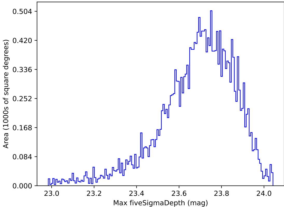
too_ignore_100_4v3.4_10yrs All sky u band: Max fiveSigmaDepth
