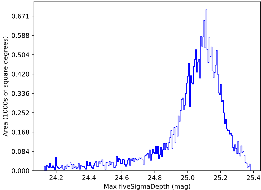
too_ignore_100_4v3.4_10yrs All sky g band: Max fiveSigmaDepth
