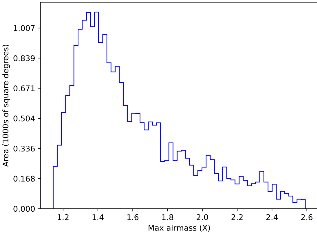
too_ignore_100_4v3.4_10yrs Yr 1 y band: Max airmass
