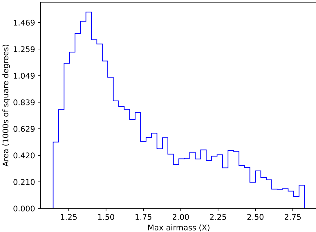
too_ignore_100_4v3.4_10yrs Yr 1 i band: Max airmass
