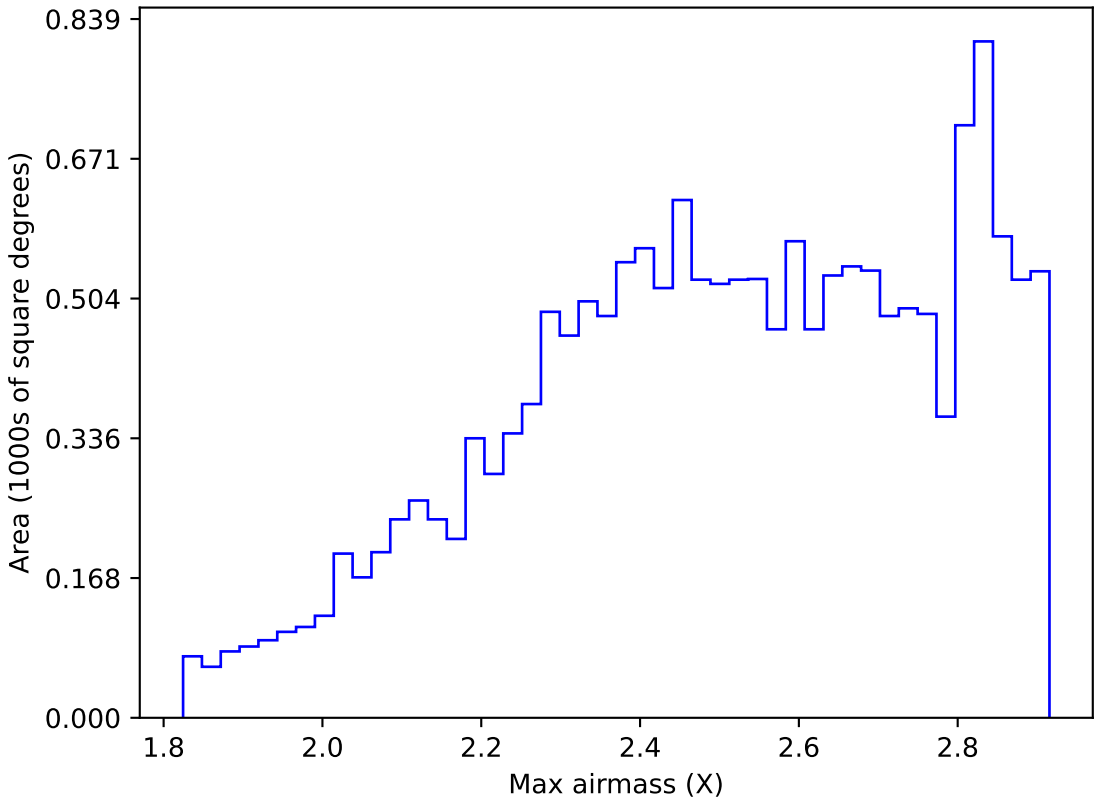
too_ignore_100_4v3.4_10yrs WFD z band: Max airmass
