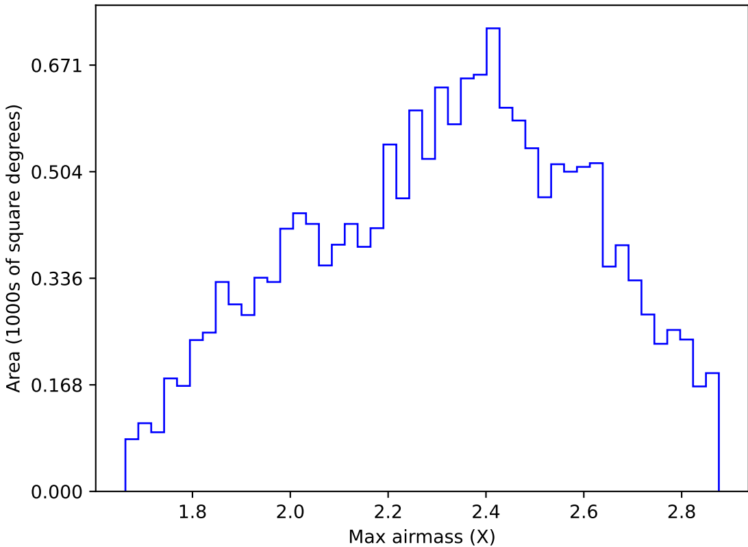
too_ignore_100_4v3.4_10yrs WFD y band: Max airmass
