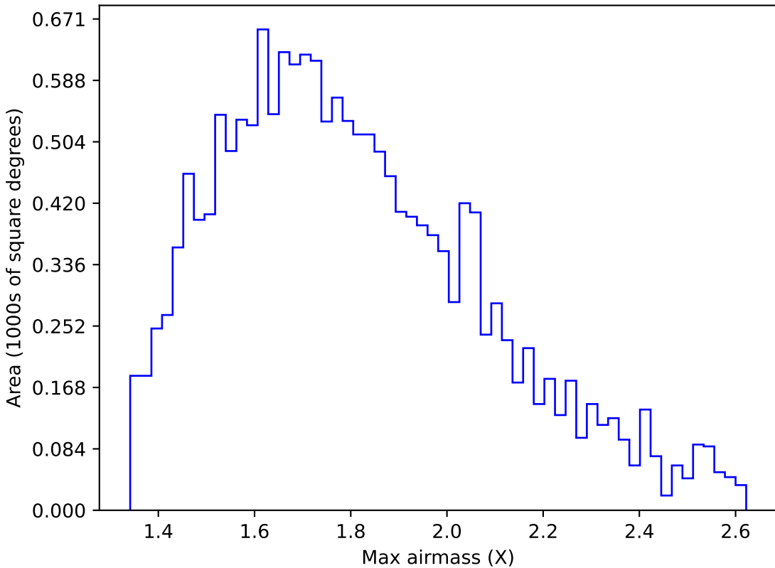
too_ignore_100_4v3.4_10yrs WFD u band: Max airmass
