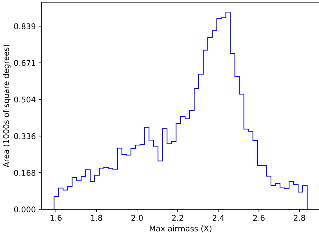
too_ignore_100_4v3.4_10yrs WFD r band: Max airmass
