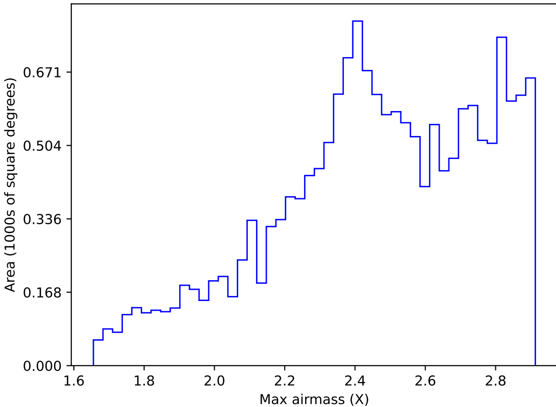
too_ignore_100_4v3.4_10yrs WFD i band: Max airmass
